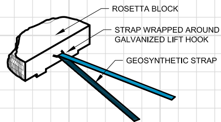
6" OR 12" HIGH ROSETTA BLOCKS
