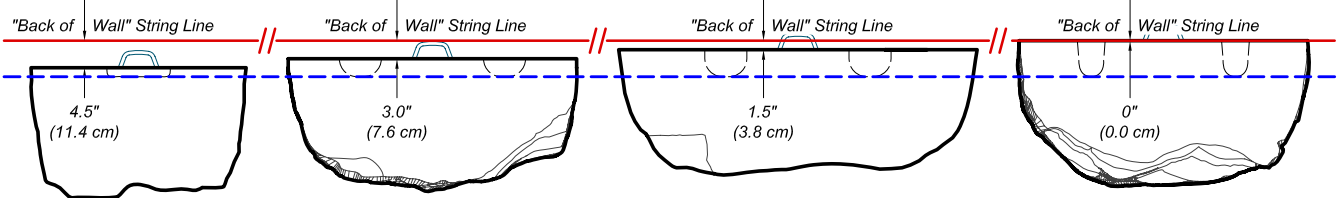
6" (15.2 cm) HIGH BLOCKS Offset Back of Block 4.5" (11.4 cm) From String Line
