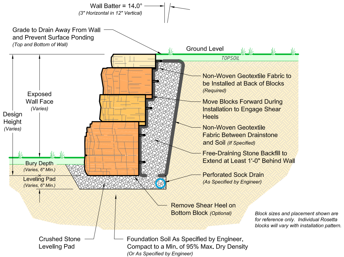
TYPICAL GRAVITY WALL SECTION (NO SCALE)
