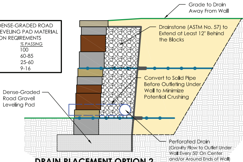
DRAIN PLACEMENT OPTION 2 THIS DETAIL IS INTENDED FOR USE WHERE GRAVITY DRAINAGE ONLY AVAILABLE TO THE BOTTOM OF THE EXPOSED WALL FACE
